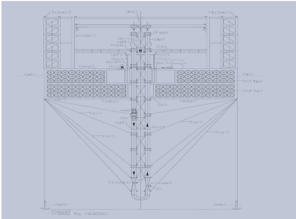
Fig. 1 shows the starting point, ie the float construction site from which arises a "floating system, hydroelectric, desalter, extractor of calcium and carbon from marine deep water". This
