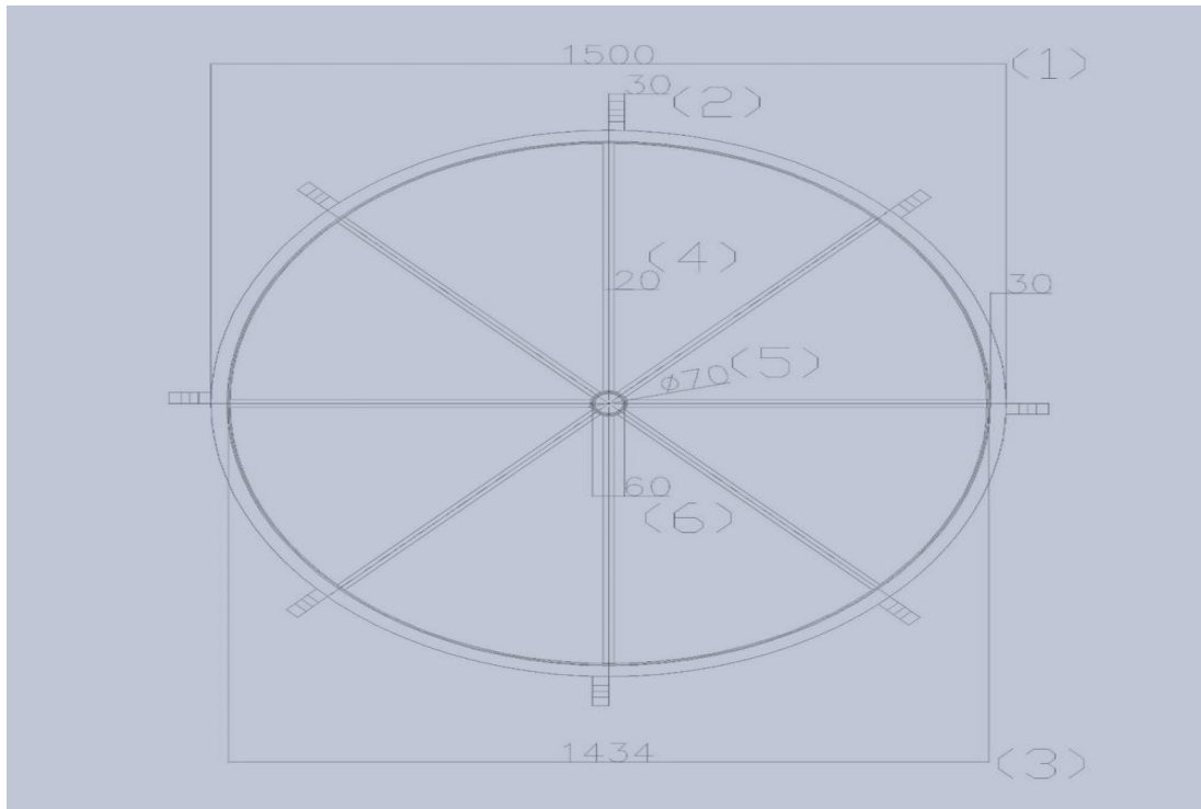
Fig. 10: (1) polyethylene pipe outside diameter 1500 mm, thickness 30 mm; (2) outer polyethylene pipe rib 80x30 with mounting holes; (3) calendered sheet 100 * 5 mm outer diameter 1434; (4) diameter steel round 20 mm; (5) smooth bore tube diameter 70 mm, lung. 80, thickness 3 mm; (6) smooth bore tube diameter 60 tickness 3 mm, length equal to the tube 1.
